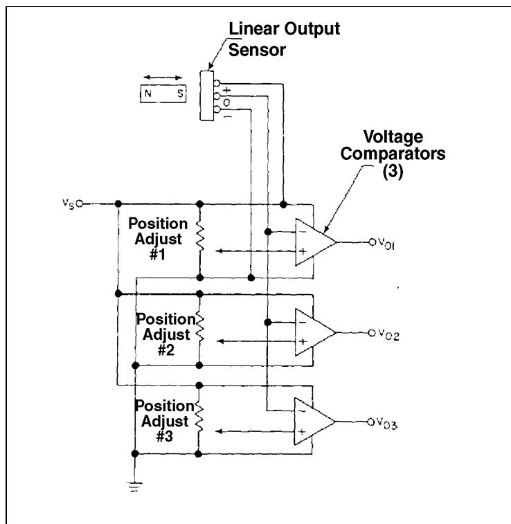
Figure 7-9 Multiple position sensor
