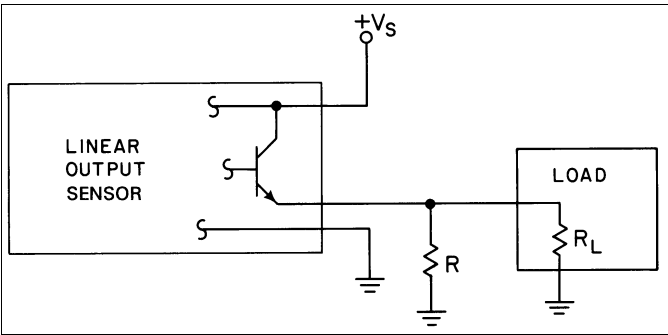
Figure 4-23 Typical load . . . Analog output sensor
