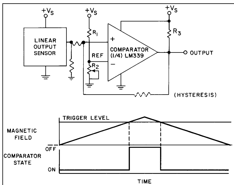
Figure 4-26 Digital system with analog sensor
