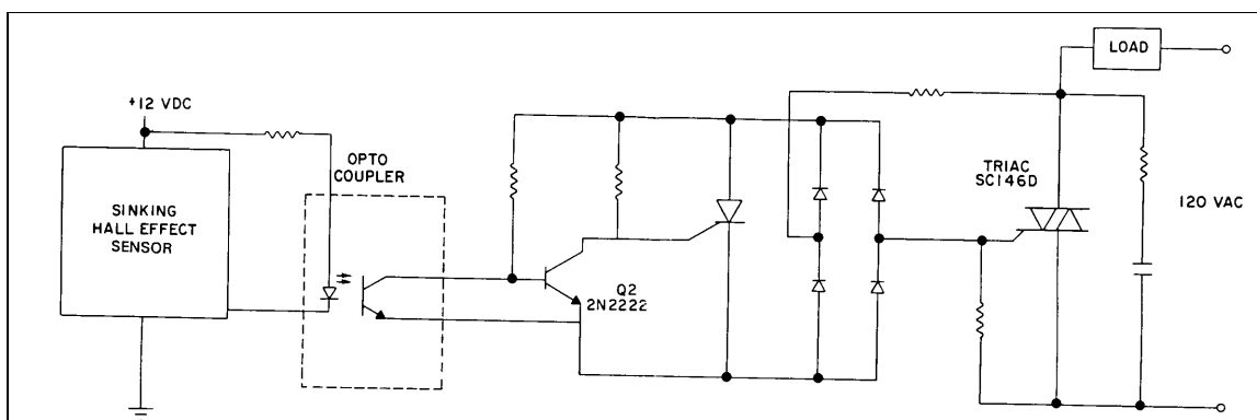
Figure 4-14 Sinking sensor interfaced to normally OFF triac
