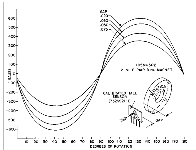
Figure C-28 Inco .625" dia. x .20" thick ring magnet
