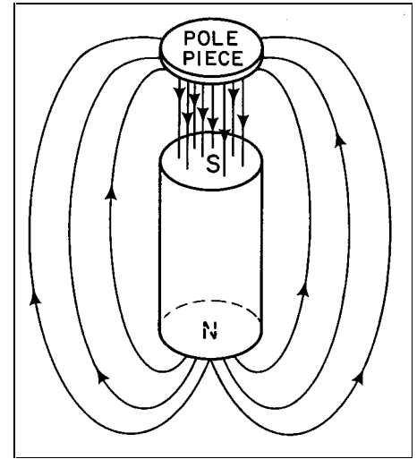
Figure 3-14 Magnet with pole pieces
