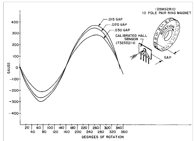
Figure C-30 Lode 42 1.75" dia. x .14" thick ring magnet
