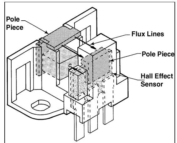
Figure 5-3 Vane operated sensor with pole pieces
