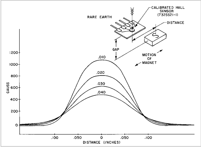
Figure C-17 Rare earth .125" x .078" x .040" thick magnet
