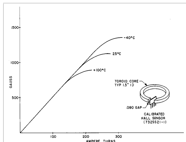
Figure C-34 Effect of temperature on typical ferrite toroid core with .080" gap
