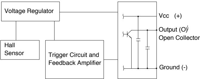
Figure 5-28 Gear tooth sensor construction and wiring diagram
