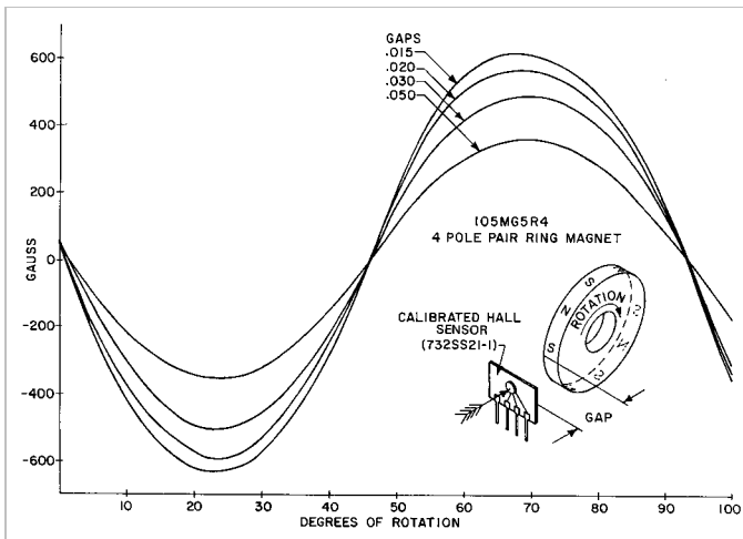
Figure C-29 Inco .625" dia. x .20" thick ring magnet
