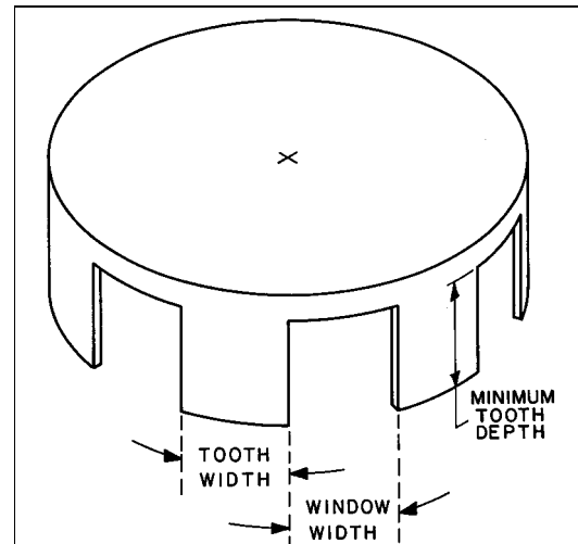
Figure 5-13 Uniform tooth and window vane
