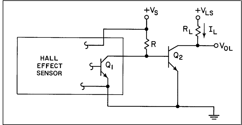
Figure 4-8 Sinking sensor - sinking output
