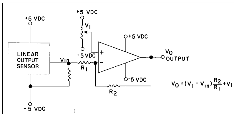
Figure 4-25 Null offset cancellation circuit
