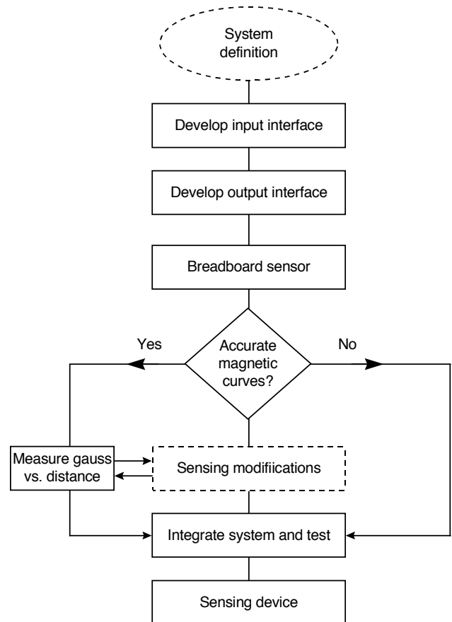
Figure 6-8 Detailed design procedure - Non-precision digital output Hall effect based sensing device
