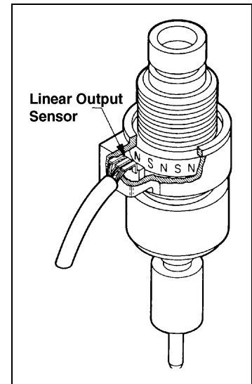
Figure 7-13 Speed sensor
