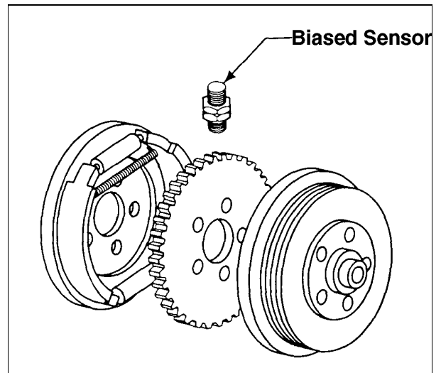
Figure 7-11 Anti-skid sensor
